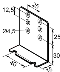
Mounting Bracket Angle Part No.: 803 799
