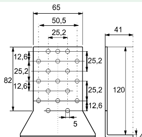
Universal Mounting Bracket Part No.: 803 798
