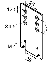
Extension Bracket Part No.: 803 800
